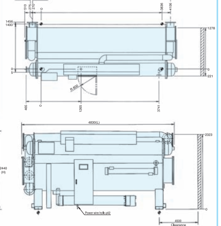
Chilled water inlet/outlet Cooling water inlet Cooling water outlet
